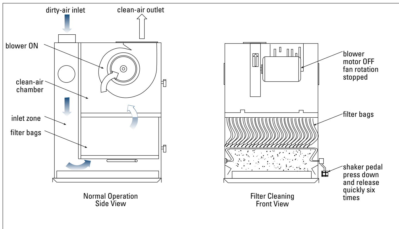
Collector Operation (Cabinet 54-84 Shown)
