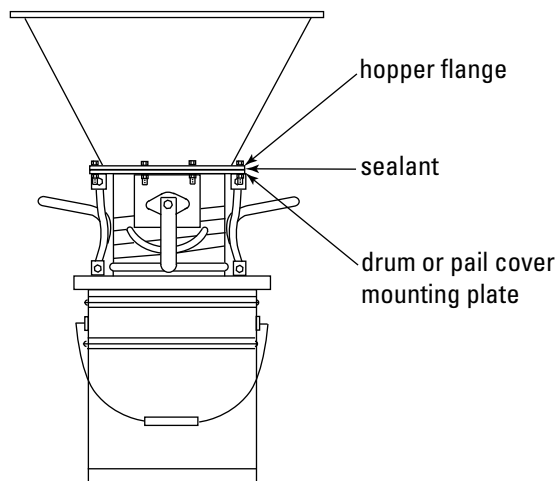
Pail Pack with Gate Valve Models 54-84 Shown
