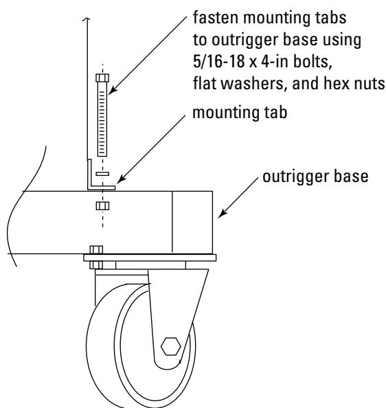
Outrigger Pack Assembly (casters are optional on models 90-3 and 90-5)
