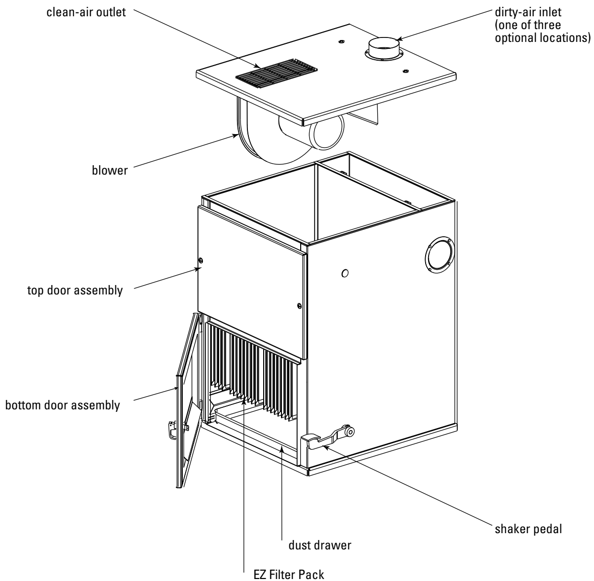
Typical Installation (Cabinet 54-84 Shown)
