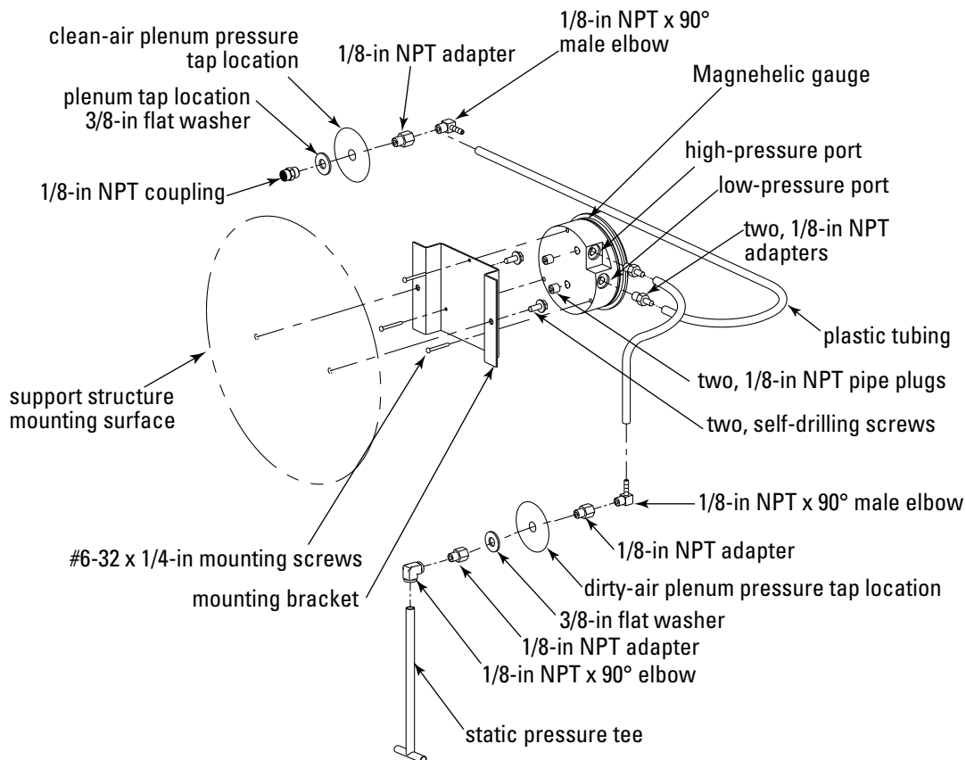
Magnehelic Gauge Assembly
