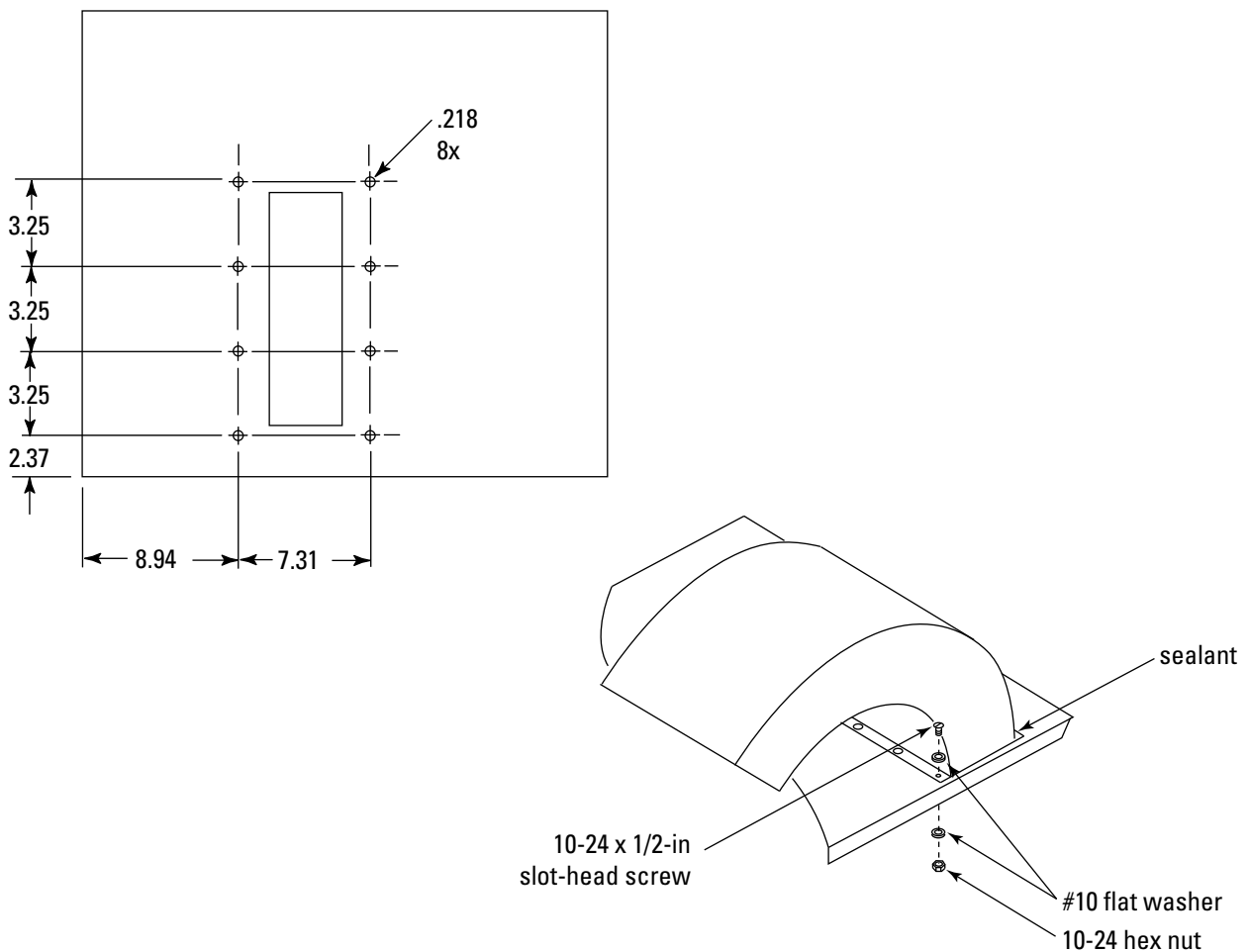
Outdoor Exhaust Deflector (only available on models 54-84)
