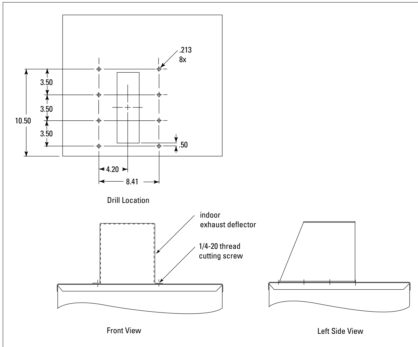
Indoor Exhaust Deflector (only available on models 54-84)
