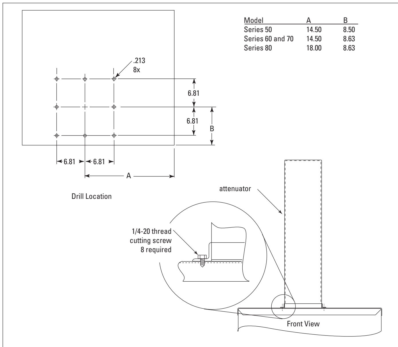
Attenuator Installation (only available on models 54-84)
