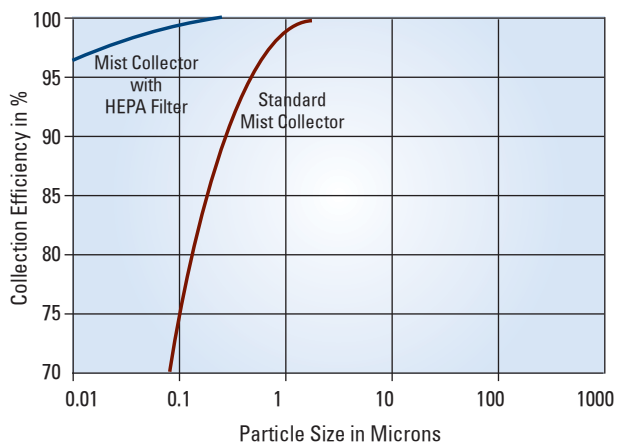
PARTICLE SIZE VS. COLLECTION EFFICIENCY
